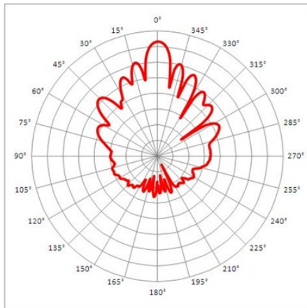
Elevation @ 2.4GHz
