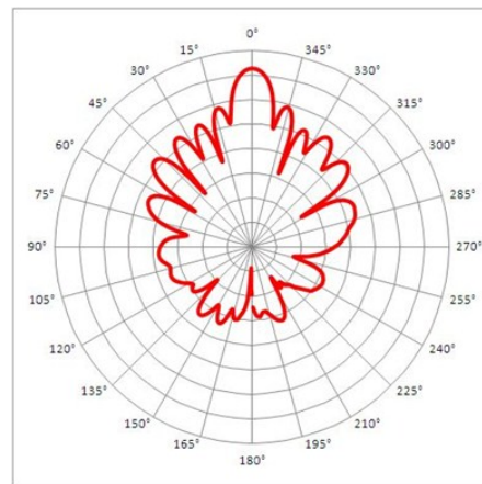
Azimuth @ 2.4GHz
